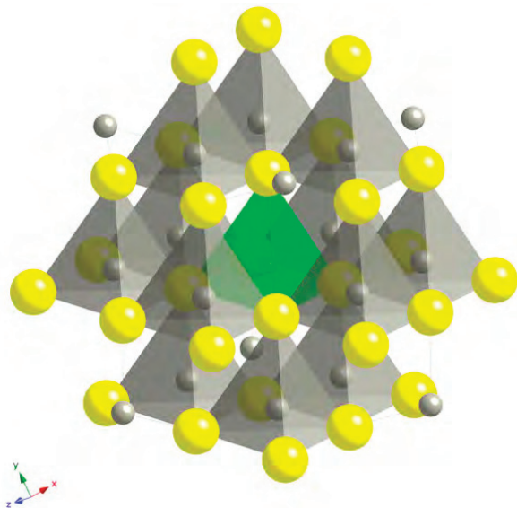
a) Cu replacing one Zn in sphalerite
