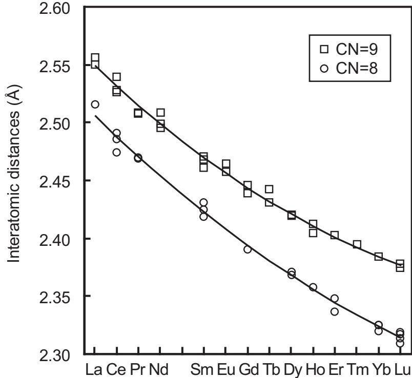
Appendix 2. Figure 1. Interatomic distances of REE compounds whose first coordination spheres are eight and nine. Solid lines indicate the fitting results using the curve of the second order.
