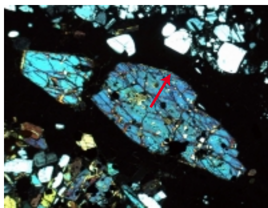
d) Fish Canyon Tuff (intracaldera)
