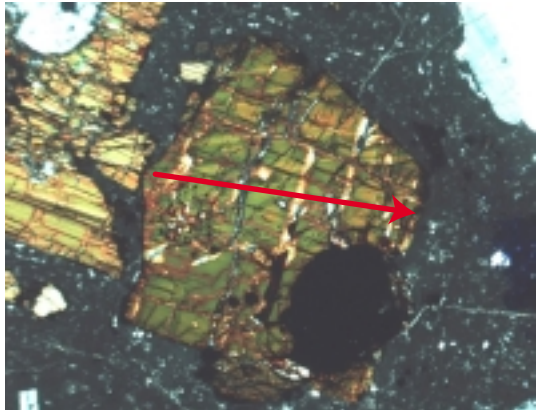
c) Fish Canyon Tuff (intracaldera)
