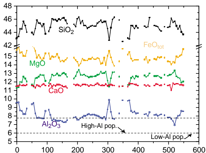
d) Fish Canyon Tuff (intracaldera)
