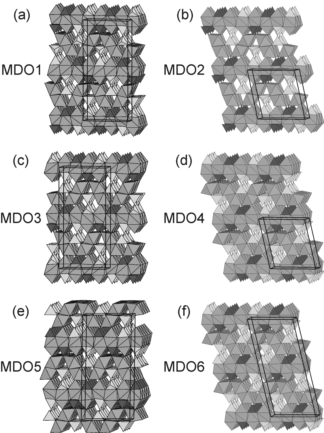
Fig. 12. Six different MDO polytypes for fukalite, as seen approximately along the silicate chain direction. The unit cells are outlined.
