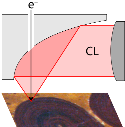
Iron (oxyhydr)oxides
