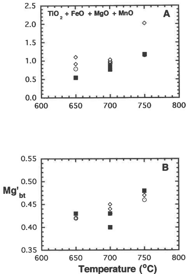
Fig. 5. (A) Feric components ( \text{FeO}_{\text{tot}} + \text{TiO}_2 + \text{MgO} + \text{MnO} ) vs. temperature in analyzed Synpel glasses. (B) \text{Mg}' [ \text{MgO}/(\text{Fe} + \text{MgO} + \text{MnO}) ] vs. temperature for experimentally grown Synpel biotites. Symbols as in Fig. 3A.
