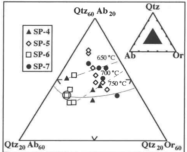
Fig. 4. Synpel melt compositions projected onto the metaluminous ternary quartz-albite-orthoclase. The 200 MPa \text{H}_2\text{O} -saturated minimum, approximately \text{Qtz}_{35}\text{Ab}_{30}\text{Or}_{35} (open circle), and the quartz-alkali feldspar cotectic (solid line) were determined by Tuttle and Bowen (1958). Symbols are as follows: solid triangles = Synpel 4, diamonds = Synpel 5, squares = Synpel 6, solid circles = Synpel 7. Note that the projected melt compositions move progressively toward the orthoclase apex with increasing temperature (dashed lines = temperature contours), reflecting increasing muscovite and biotite melting.
