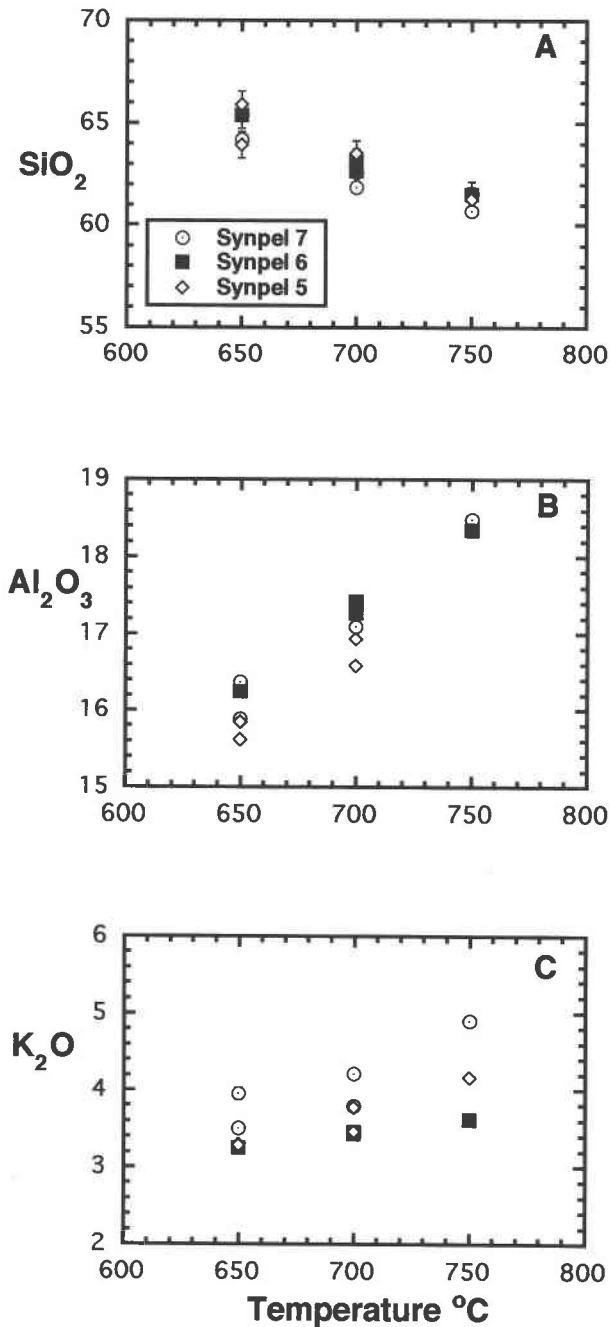
Fig. 3. Compositions of analyzed glasses (quenched melt) in the experimental charges. Symbols are as follows: diamonds = Synpel 5, squares = Synpel 6, circles = Synpel 7. Error bars represent 1\sigma errors, as described in the Appendix. (A) \text{SiO}_2 vs. temperature. Silica is highest at low temperature where quartz is lost from the starting assemblage. (B) \text{Al}_2\text{O}_3 vs. temperature. Melting of white mica and continuous reaction of biotite with melt both contribute Al to melt. (C) \text{K}_2\text{O} vs. temperature. The rise in Al with temperature, as seen in B, is offset by a concomitant rise in K that keeps the ASI \leq 1.4 .
