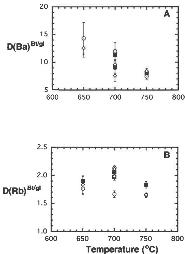
Fig. 10. Temperature dependence of distribution coefficients: (A) D(\text{Ba})^{\text{Bt/gf}} shows a strong decrease with increasing temperature. (B) D(\text{Rb})^{\text{Bt/gf}} shows no correlation with temperature. Error bars represent 1\sigma errors. Symbols as in Fig. 3A.
