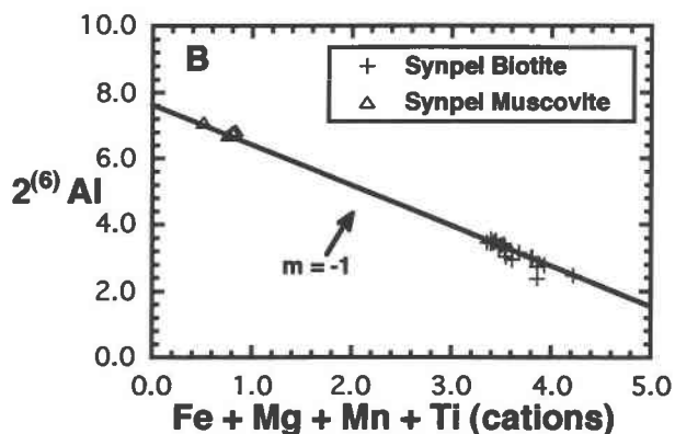
Fig. 9. (A) Proposed substitution mechanism for Ba into Synpel biotite and white mica (muscovite): 112 Ba 2+ + 64 Al 3+ = 14 Si 4+ + 112 (K + Na + Cs + Rb) 1+ (in cations). (B) Proposed substitution mechanism for Ti in octahedral sites into Synpel biotite and white mica: 161 Ti 4+ + 161 (Mg + Mn + Fe) 2+ = 2 61 Al 3+ (in cations).
