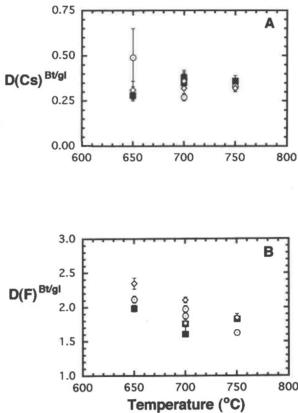
Fig. 11. Temperature dependence of distribution coefficients: (A) D(\text{Cs})^{\text{Bt/gf}} shows no correlation with temperature. (B) D(\text{F})^{\text{Bt/gf}} shows a decrease with increasing temperature. Error bars represent 1\sigma errors. Symbols as in Fig. 3A.
