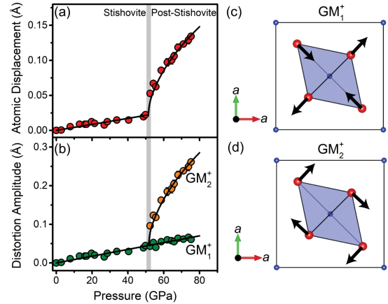
FIGURE 5. Atomic displacements and distortion mode amplitudes across the post-stishovite transition at high pressure. (a) Maximum displacement of O atoms in the crystal structure; (b) Amplitude of \text{GM}_1^\dagger and \text{GM}_2^\ddagger distortion modes. Black lines are best linear or polynomial fits to guide the eyes. Atomic displacements for \text{GM}_1^\dagger and \text{GM}_2^\ddagger are schematically drawn in c and d, respectively. In c and d, blue and red spheres represent Si and O atoms, respectively, shaded area represents a \text{SiO}_6 octahedron, and black lines with arrows represent atomic displacements upon compression.
