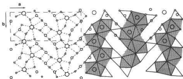
Fig. 1. Schematic diagram of the sartorite structure showing the chains of \text{PbS}_3 polyhedra parallel to \mathbf{b} , which are cross-linked by strips of \text{AsS}_3 polyhedra in a twinned or zig-zag arrangement. The \text{PbS}_3 chains, similar to those found in \text{PbCl}_2 , are shaded. The structure is viewed down [001] . Pb, large circles; As, medium circles; S, small circles.
