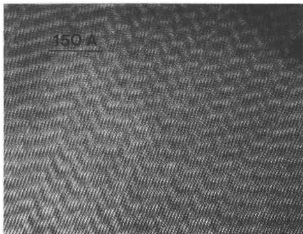
Fig. 9. Lattice image of sartorite down [010] showing domains of ordered twinning of the structural modulation, which range from 50 up to 150 Å in width.
