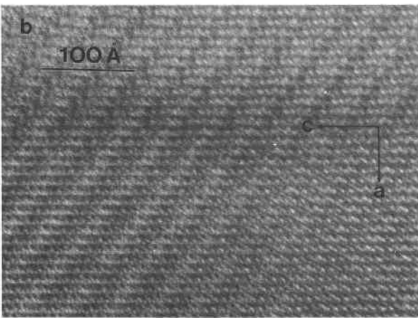
Fig. 4. Electron diffraction pattern and lattice image of sartorite taken down [010]. (a) The electron diffraction pattern shows an apparently incommensurate superlattice, which runs approximately along (15.0.4)^* with a real space period of 32.4 \text{ \AA} . This pattern is generated by a rotation of \mathbf{q}^{\text{prim}} 3^\circ away from (101)^* toward (001)^* . The value of \mathbf{q}^{\text{prim}} is again \approx 6/13(101)^* ; the higher harmonics m\mathbf{q} are labeled. (b) Corresponding lattice image showing contrast modulations due to the incommensurate modulation in the structure.
