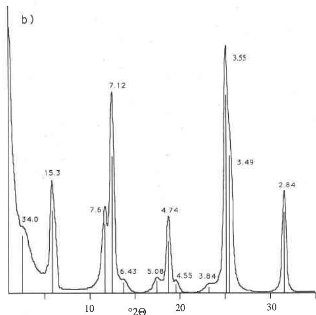
Fig. 4. Calculated glycolated XRD patterns for chlorite/smectite (65:35) and chlorite (Reynolds, 1985). (a) Pattern for a regular mixed-layer tri-chlorite/tri-smectite 2-glycol with 65% chlorite content. (b) Pattern for a physical mixture between a discrete tri-chlorite and a tri-chlorite/tri-smectite 2-glycol mixed-layer mineral in the respective abundances of 55 and 45%, with the proportion of chlorite in the mixed-layer mineral at 65%.
