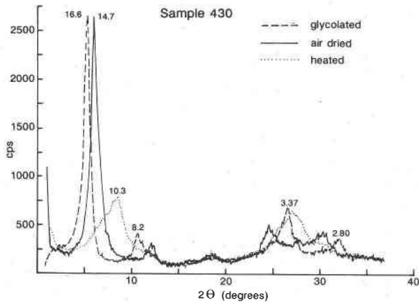
Fig. 6. XRD patterns for sample 430, for air-dried state, glycolated, and heated to 315 °C. The pattern is representative of a virtual monomineralic random mixed-layer chlorite/smectite (25:75).
