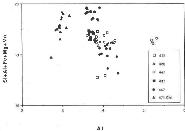
Fig. 7. Noninterlayer (Si + Al + Fe + Mg + Mn) cation total vs. Al_{10t} for samples with only chlorite (samples 413, 426, and 447 = open symbols); chlorite + second phyllosilicate phase (closed symbols), which include chlorite + celadonite (samples 437 and 467), and chlorite + random mixed-layer chlorite/smectite (sample 471-Chl). This figure and all subsequent figures show analyses plotted on the basis of a chlorite formula with 28(O,OH) .
