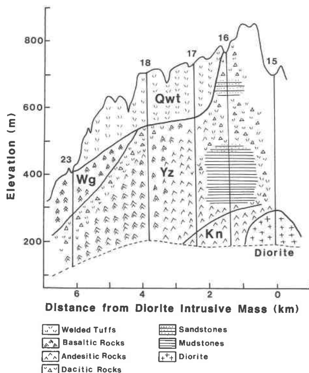
Fig. 2. Geologic cross section along the line of Figure 1. Qwt = Quaternary welded tuffs; Wg = Wadagawa formation; Yz = Yotsuzawa formation; Kn = Kanezawa formation.
