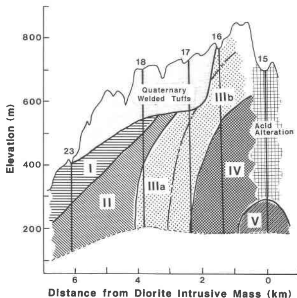
Fig. 3. Cross section showing the distribution of zones.
