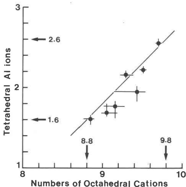
Fig. 7. Plot of [ IV Al] content vs. total of octahedral cations per O 20 (OH) 10 in corrensite. Bars indicate ranges of data. The solid line indicates the correlation of Fe-rich corrensite as noted by Inoue (1985).
