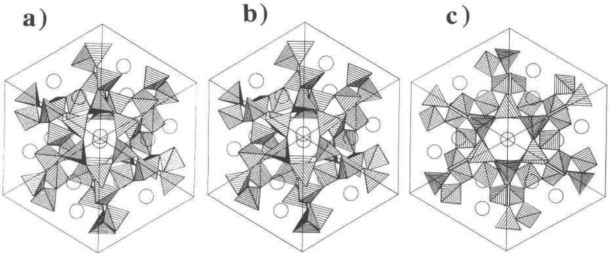
Fig. 4. Projection down [1\bar{1}\bar{1}] of the structure of leucite: (a) observed tetragonal structure at room temperature, (b) calculated tetragonal structure, (c) observed cubic structure. The comparison of a and b shows that our model has reproduced the tetragonal distortion from c. Observed structure data are from Dove and Palmer (in preparation).
