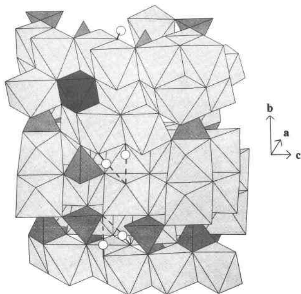
Fig. 4. The three dimensional structure of phase B showing the relative positions of the H atoms, which are indicated by small circles.
