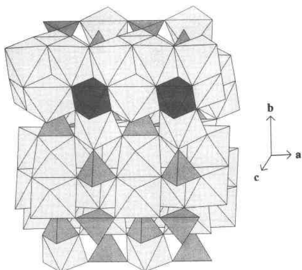
Fig. 3. The three dimensional structure of phase AnhB showing the cross linkages.
