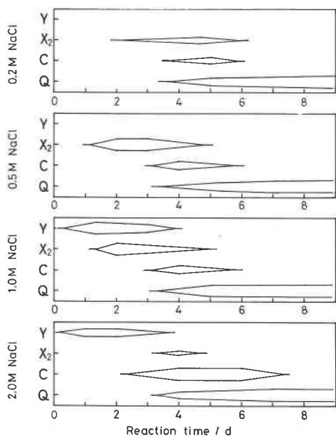
Fig. 1. Effect of NaCl concentration in 1% KOH solution in the composition of \text{SiO}_2\text{:OH}^-:\text{Na}^+ = 3:1:1.1\text{--}11.0 at 160 °C on the crystallization sequence of \text{SiO}_2\text{-Y} (Y), \text{SiO}_2\text{-X}_2 ( \text{X}_2 ), cristobalite (C), and quartz (Q) as a function of reaction time.
