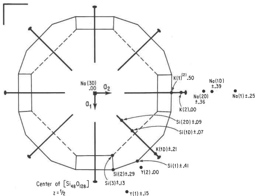
Fig. 2. The central ball drawn as [\text{Si}_{48}] connections, with mirror planes and twofold and fourfold rotors drawn in. The linking oxygen atoms are approximately at the midpoints of the "edges." The breaks of the edges for the truncated cuboctahedron are shown as dashed lines. There are eight such dashed lines, each representing two oxygens instead of one such that \text{Si}_{48}\text{O}_{120} + \text{O}_8 = \text{Si}_{48}\text{O}_{128} . Surrounding cations in the border or limbus and cations in the disordered why are also shown, heights as fractional coordinates in z following Table 3.
