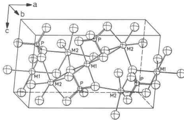
Fig. 4. ORTEP computer drawing of the sarcopside structure, showing an (M2) \text{O}_6 -(M1) \text{O}_6 -(M2) \text{O}_6 trimer of edge-sharing octahedra.
