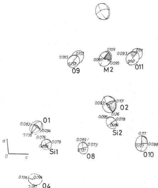
Fig. 4. Projection of magnitude and orientation of principal axes of M(2), Si(1), and Si(2) sites on the (010) plane. Root-mean-square thermal displacements (Å) are shown.
