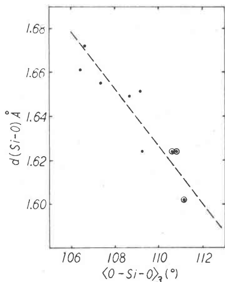
Fig. 5. Pumpellyite, scatter diagram of the observed Si-O bond lengths ( d(\text{Si-O}) ) plotted against the average of the three O-Si-O angles common to each bond ( \langle \text{O-Si-O} \rangle_3 ) after Wan et al. (1977).
