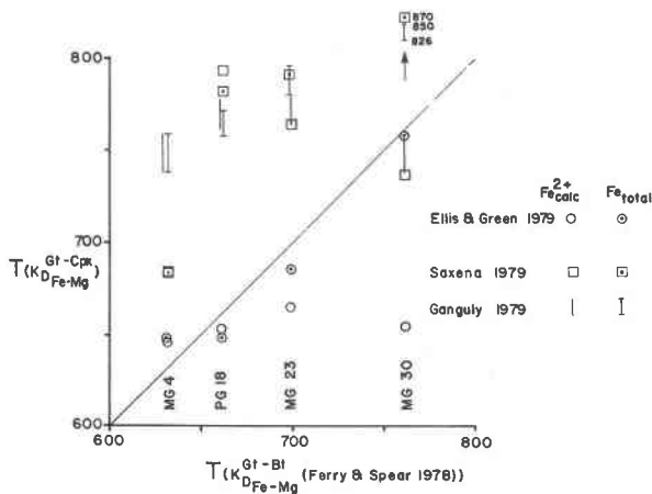
Fig. 7. Comparison of temperature estimates derived from garnet-biotite and various garnet-clinopyroxene thermometers. The two thermometers are consistent if the Ferry and Spear (1978) and Ellis and Green (1979) calibrations are used and K_D is calculated using the total iron content rather than stoichiometrically-determined Fe^{2+} .
