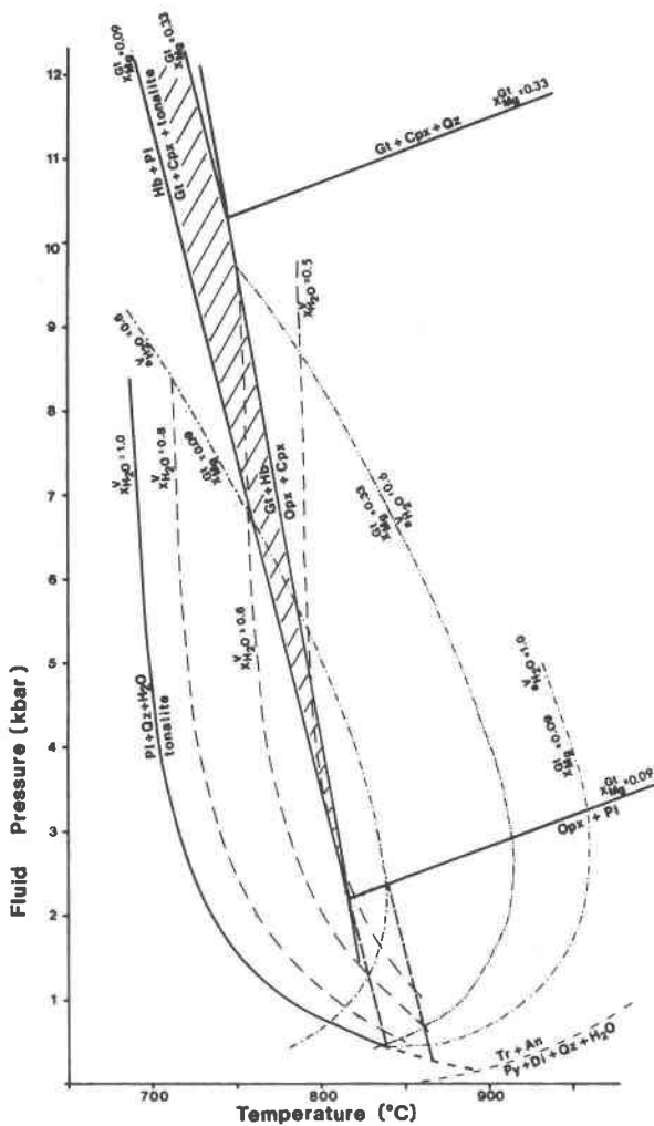
Fig. 5. Vapor-phase-absent-melting curve (diagonal ruling) corresponding to the reaction Hb + Pl = Gt + Cpx + tonalite for mafic rocks of variable Mg/(Mg+Fe) ratio. The curve is defined by the locus of intersection between dehydration (Reaction 2; dot-dash symbol) and melting (Kilinc, 1979) curves of equal water activity. Position of curves for reaction Opx + Pl = Gt + Cpx + Qz at variable X_{Mg}^{Gt} are based on Hansen (1981; p. 239) Symbols as for Fig. 3 except Py: pyrope; Tr: tremolite; Di: diopside; An: anorthite.
