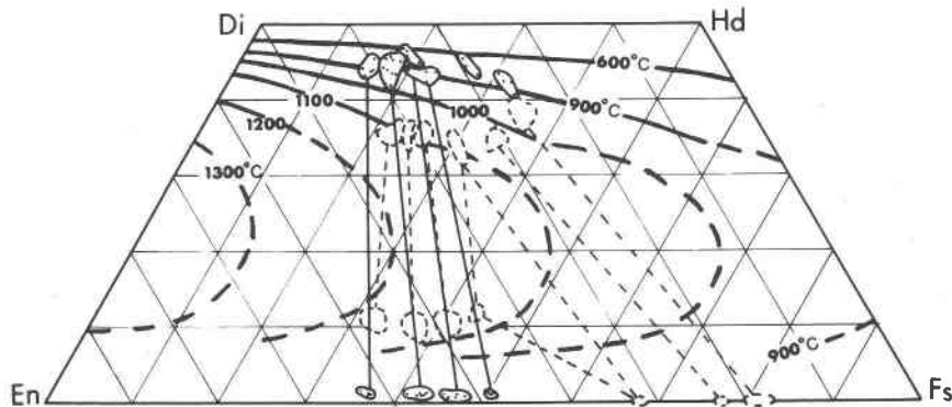
Fig. 3 (A) Primary pyroxene compositions as determined using broad beam energy dispersive techniques, and olivine compositions as determined using wavelength dispersive analyses. Solid tie lines: mafic cumulate layers. Dashed tie lines: mafic dikes. Skaergaard trend after Wager and Brown (1968). (B) Compositions of primary igneous pyroxene and pyroxene-olivine pairs (short dashed lines) and reconstituted metamorphic pairs (solid lines) plotted with respect to the augite-pigeonite solvus (dashed contours) and the augite orthopyroxene solvus (solid contours) of Ross and Huebner (1975).
