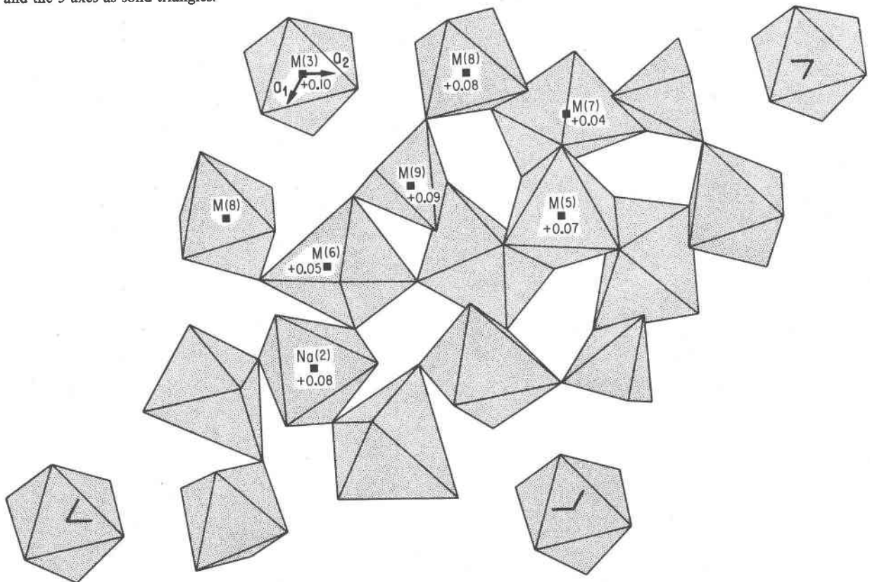
Fig. 2b. Conventional projection of the slab at z = 1/12 showing only the larger polyhedra. Atoms in the asymmetric unit with heights in z are labelled. \text{M}(3) , \text{M}(6) , \text{M}(7) , \text{M}(9) and \text{Na}(2) are octahedra; \text{M}(6) and \text{M}(9) are five-coordinated.
