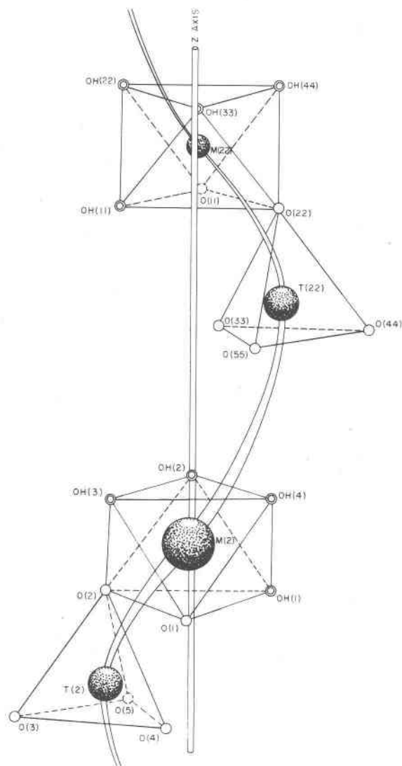
Fig. 2. Tetrahedra and octahedra enclosing Al atoms spiral along lines that parallel the Z axis. In this figure the Y axis is horizontal and lies in the plane of the page. The +Z axis is tilted 10° out of the plane of the page toward the reader. The relative sizes of the Al atoms indicate distance, with M(2) closest to the reader and M(22) farthest away.
