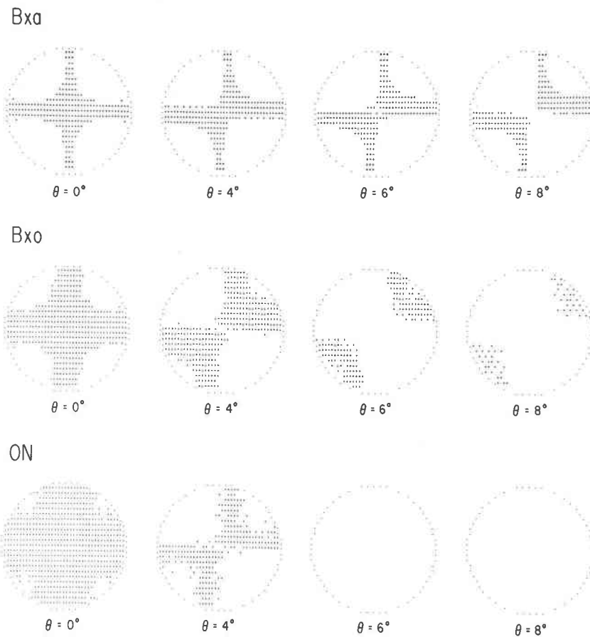
Fig. 8. Computer-generated orthoclase Bxa (top row), Bxo (center row), and ON (bottom row) figures through clockwise stage rotation ( \theta ).
