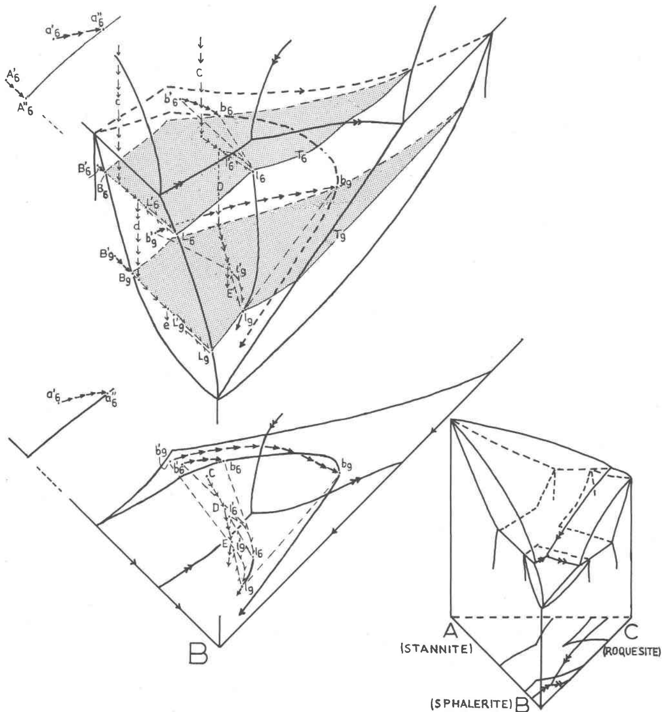
Fig. 9. Perspective sketch of equilibrium diagram, showing course of oscillatory crystallization and fractional crystallization in a ternary system with limited solid solution and peritectic relationships between components; A may represent stannite, B sphalerite, and C roquesite. See text for further explanation.
