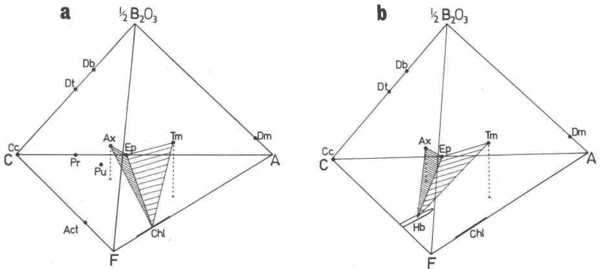
Fig. 6. ACF- B_2O_3 quaternary diagrams, assuming excess SiO_2 and H_2O are completely mobile (see text for explanation). (a) Compositional relationships between the borosilicates axinite (Ax), tourmaline (Tm), danburite (Db), datolite (Dt), and dumortierite (Dm) and metamorphic phases typical of the prehnite-pumpellyite, pumpellyite-actinolite, and chlorite zone greenschist facies. (Cc = calcite, Pr = prehnite, Pu = pumpellyite, Act = actinolite, Ep = epidote, Chl = chlorite). (b) Mineral assemblages reported in the biotite and garnet zones, greenschist facies and the amphibolite facies. Hornblende (Hb) is the stable amphibole phase. Other abbreviations as in 6a.
