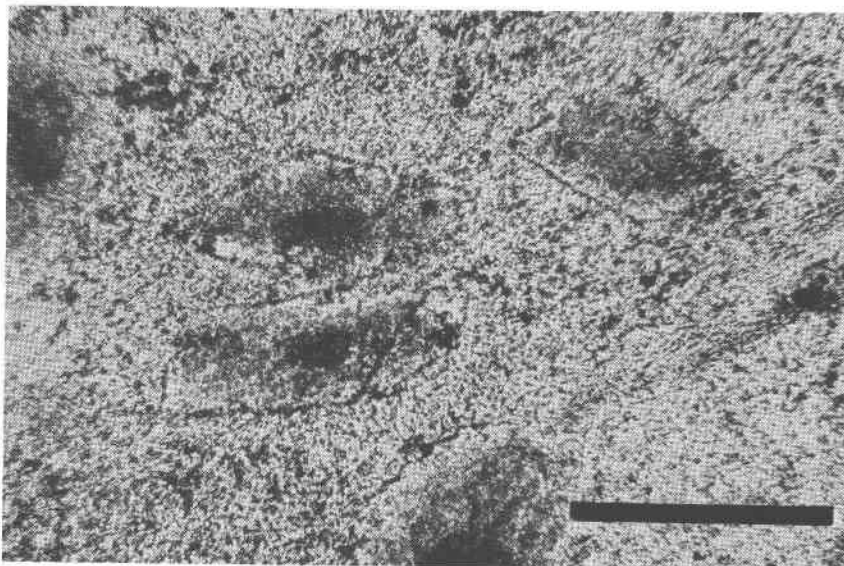
Fig. 3. Manganaxinite porphyroblasts in OU 44672. Minute inclusions of quartz and hematite are concentrated in grain cores. The fine-grained groundmass consists of quartz, ferrostilpnomelane, manganooan ripidolite, and minor spessartine. Scale bar is 250 \mu\text{m} .
