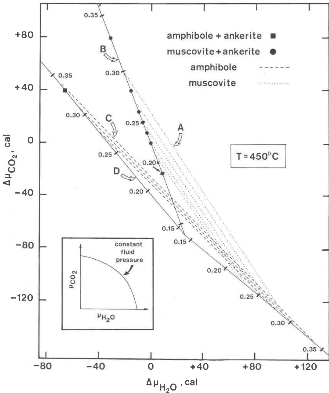
Fig. 6. Quantitative isobaric, isothermal \Delta\mu_{\text{CO}_2}-\Delta\mu_{\text{H}_2\text{O}} diagram representing selected equilibria from Figure 5. \Delta\mu_i = (\mu_i)_{\text{sample}} - (\mu_i)_{5-3} , i.e., the scale is relative to sample 5-3 ( 0 \mu_{\text{CO}_2} , 0 \mu_{\text{H}_2\text{O}} ). The origin is arbitrarily positioned and as such has no particular significance. Positioning of curves and their segmentation by composition described in the text. The curves are segmented and labeled with values of the composition variable X_{\text{FeCh}} . Circles are assemblage type (b); square, assemblage type (d); dotted lines, assemblage type (a); dashed lines, assemblage type (c). Inset illustrates the shape of the loci of points corresponding to a C-O-H-S fluid of constant fluid pressure coexisting with graphite and pyrrhotite of constant composition. Plotted assemblage types are those in Table 3.
