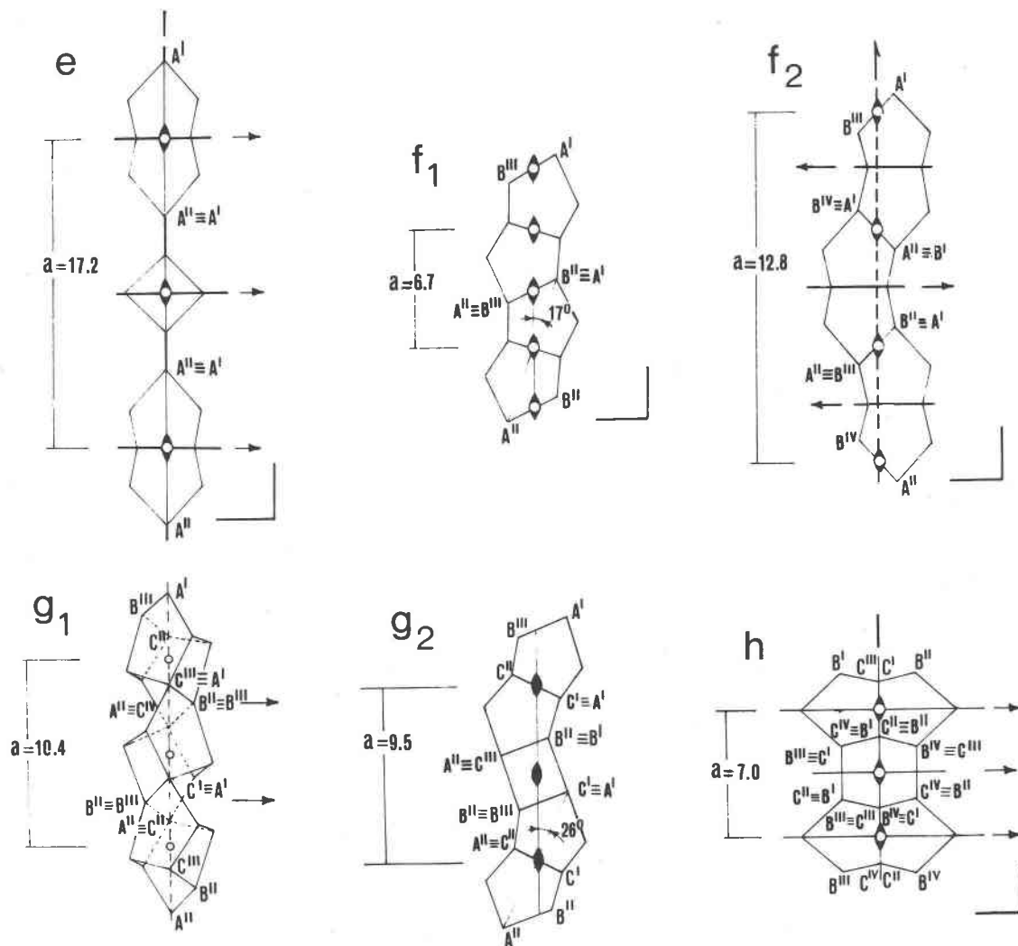
Fig. 2. Possible chains with a period repeated not more than every two units, and approximate parameters.
