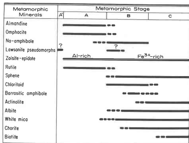
Fig. 3. Schematic paragenetic diagram illustrating mineral assemblages and metamorphic stages in the Zermatt-Saas and Combin metabasites from the Breuil-St. Jacques area. Dashed lines signify rare or questionable occurrences. The persistence of metastable relics is not shown. Stages A, B, and C are all preserved in rocks of the Zermatt-Saas unit, whereas the Combin prasinities, which contain rare relict sodic amphiboles as well as minor hornblende amphiboles, reflect dominantly stage-C recrystallization. It is not clear whether the hypothesized production of lawsonite (now represented by zoisite-epidote + white mica prismatic intergrowths) occurred prior to stage A, or during stage B, or both.
