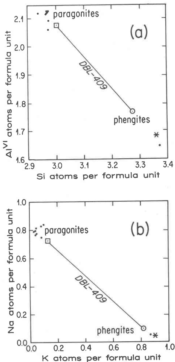
Fig. 8. Atomic proportions based on 12 anions of (a) \text{Al}^{\text{VI}} vs. Si, and of (b) Na vs. K for white micas from Breuil-St. Jacques eclogitic and other mafic rocks. The coexisting paragonite (open square) + phengite (open circle) pair analyzed from sample DBL-409 is also shown. The starred sample is from the Combin unit, all others being from the Zermatt-Saas unit.
