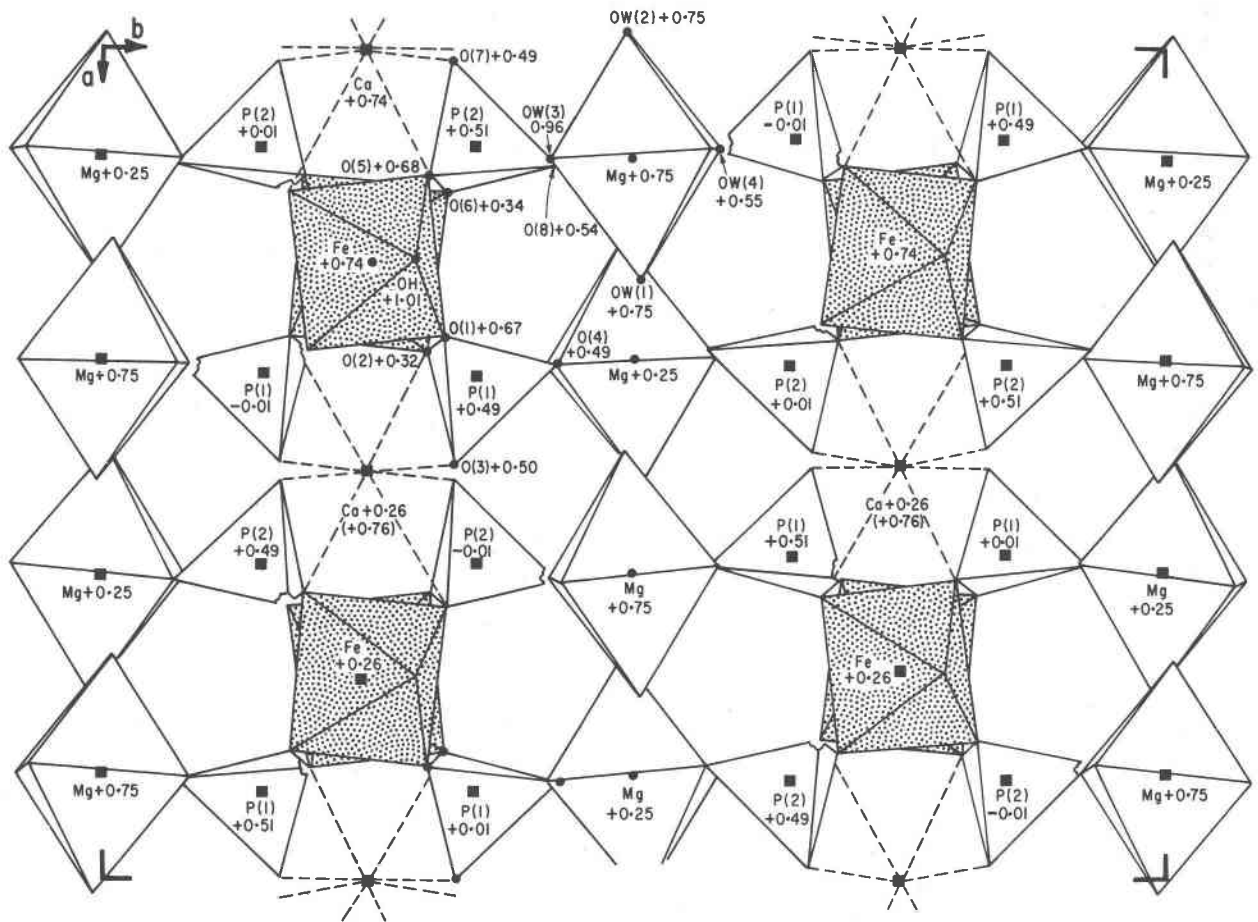
Fig. 3. The real segelerite structure projected down [001]. Note the bridging Mg-O octahedra and the compact [\text{Ca}_2\text{Fe}_3^+(\text{OH})_2(\text{PO}_4)_4]^{4-} slabs. Heights are given as fractional coordinates in z .
