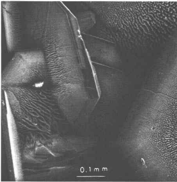
FIG. 5. Scanning electron micrograph of offretite overgrowths on levyne from Queen Creek, near Superior, Arizona. Note that the offretite fibers have grown only on the basal faces of the levyne.
