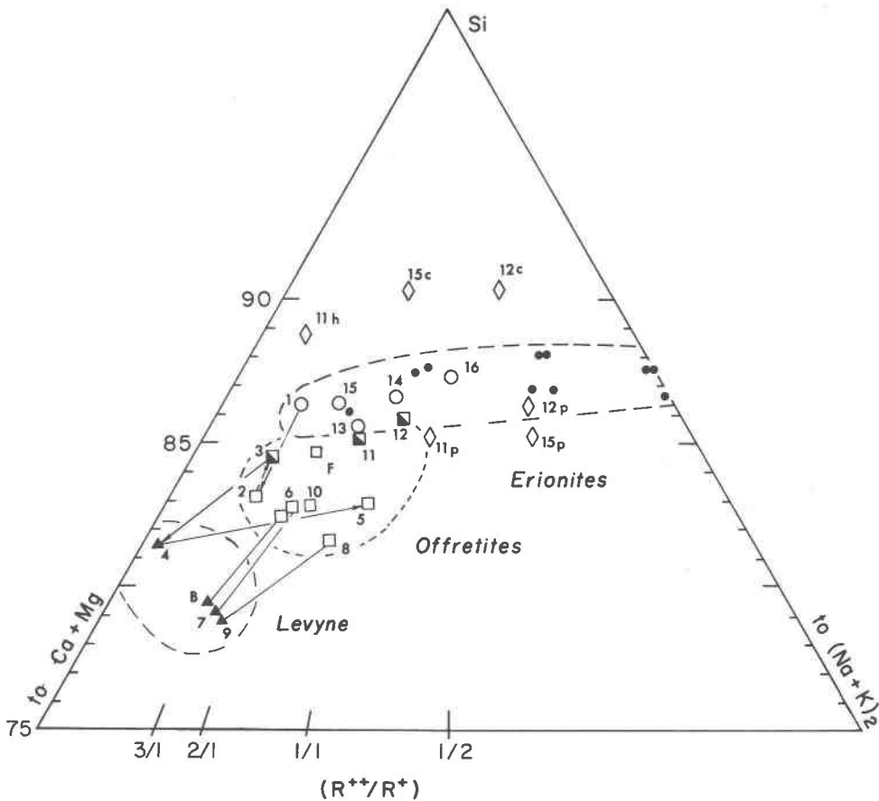
FIG. 9. Plot of Si-(Ca + Mg)-(Na 2 + K 2 ) of the analyzed minerals in Table 1. Numbers correspond to analyses. Circles are erionites (solid circles are from Sheppard and Gude, 1969), squares are offretite (half-filled squares are intergrowths of offretite and erionite). Triangles are levynes. Arrows connect the growth sequence of the Milwaukie intergrowths, and lines connect the offretite overgrowth with the host levyne. Sample B is Beech Creek, Oregon, offretite-levyne (Sheppard et al. , 1974); Sample F is original offretite, Montbrison, France (Sheppard and Gude, 1969). Diamonds labeled p , h , or c indicate associated phillipsite, heulandite, or clinoptilolite, respectively.
