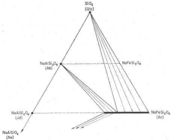
FIG. 1. Schematic isothermal, isobaric diagram for a portion of the system \text{SiO}_2\text{-NaAlSi}_3\text{O}_8\text{-NaFeSi}_3\text{O}_8 . The join \text{NaAlSi}_3\text{O}_8\text{-NaFeSi}_3\text{O}_8 was investigated in this study.
