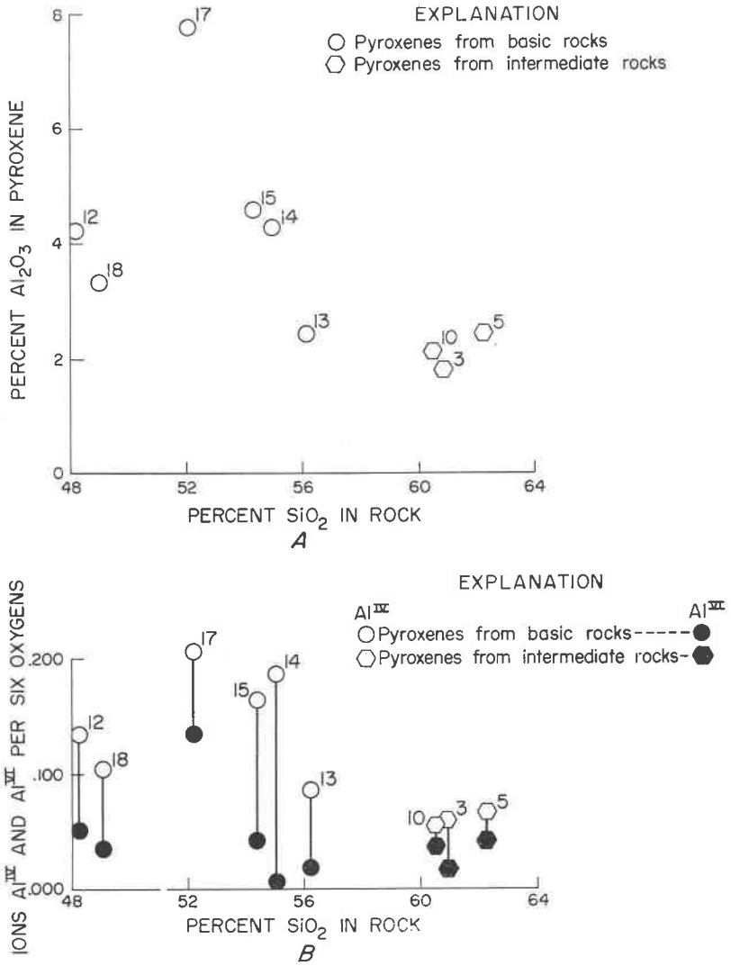
FIG. 2. Variation diagrams. A. Plot of percentage of \text{Al}_2\text{O}_3 in pyroxenes versus percentage of \text{SiO}_2 in rocks. B. Plot of \text{Al}^{\text{IV}} and \text{Al}^{\text{VI}} ions (on basis of six oxygens) versus percentage of \text{SiO}_2 in rocks.
