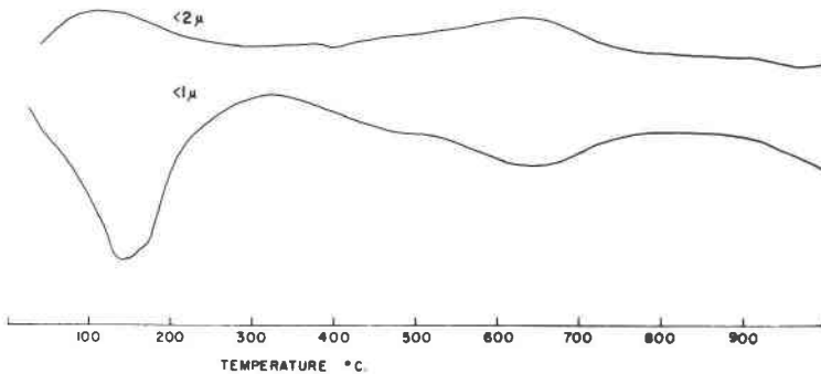
FIG. 3. Differential Thermal Analysis patterns of Mound Lake glauconitic mica. Equilibrated over saturated \text{CaCl}_2 solution, relative humidity 30%.
