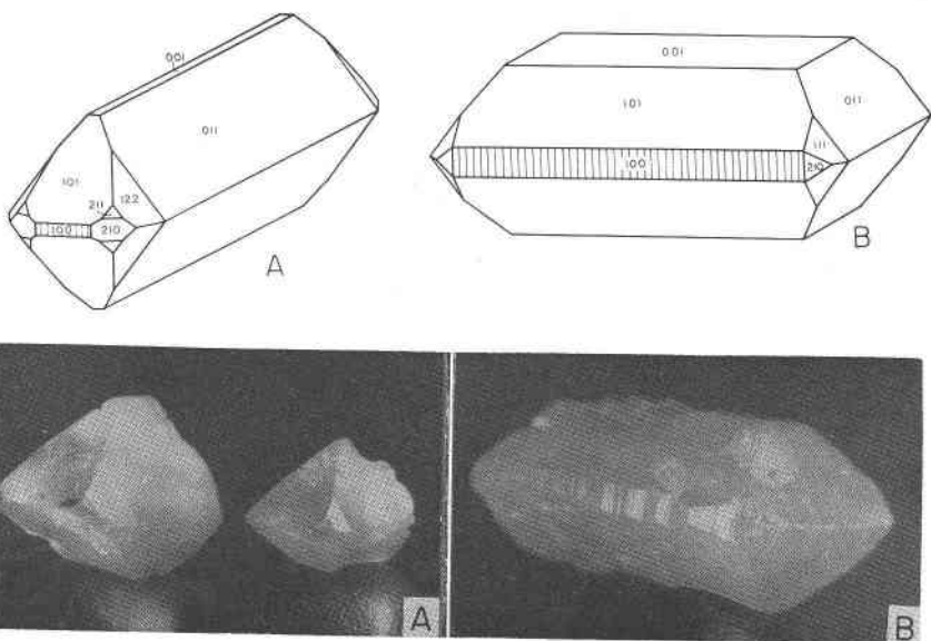
FIG. 1 (above). Idealized drawings of the two habits exhibited by celestite crystals from Wise County, Virginia.
