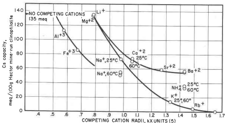
FIG. 11. The effect of competing cations on the Cs capacity of clinoptilolite. The point for Cs + at 0 Cs capacity is theoretically correct because Cs cannot compete with itself.
