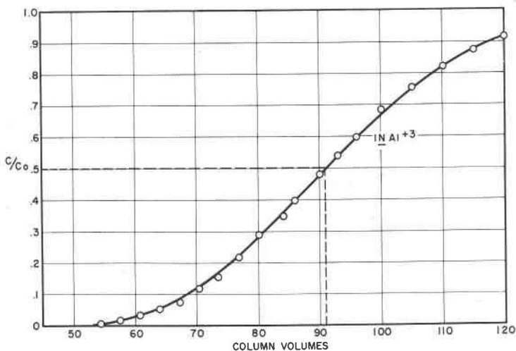
FIG. 2. Cesium Breakthrough Curve with Competing 1N\text{ Al}^{+3} .
