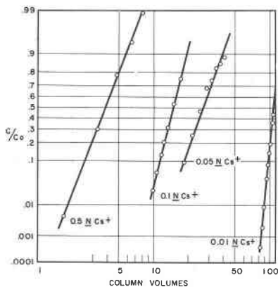
FIG. 4 (left). The Variation of Clinoptilolite Cs Capacity with Cs Concentration.
