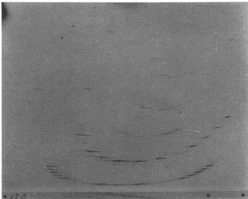
FIG. 5(c). First layer Weissenberg photograph. Rotation about [1\bar{1}0] for area with 2V=3^\circ .
