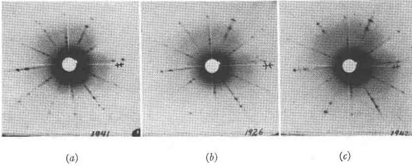
FIG. 4. Laue photographs.
