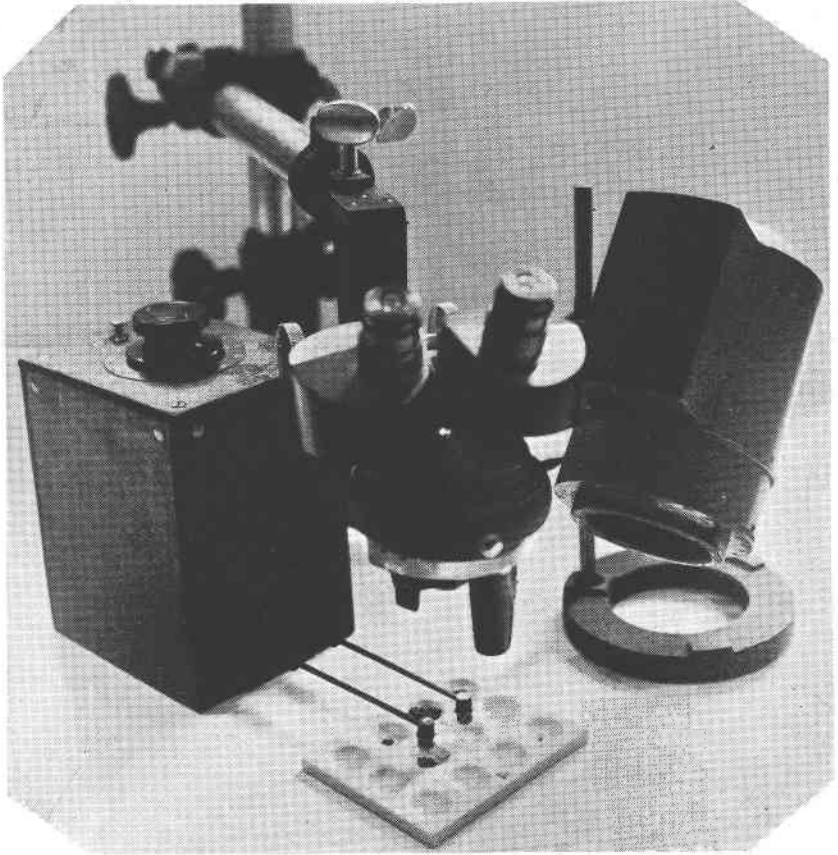
FIG. 1. Electrically-heated platinum wire in use.
