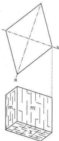
FIG. 1. Plan and clinographic projection of augelite cleavages m\{110\} and x\{101\} . FIG. 2. Optical orientation diagram of augelite. Section parallel to \{010\} .
