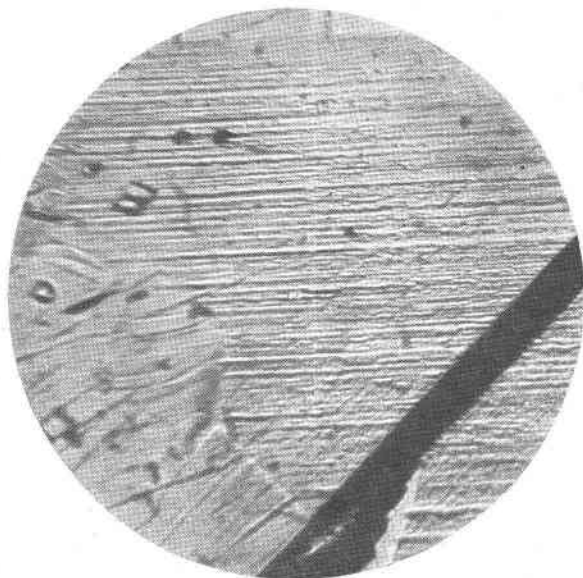
FIG. 4. Parallel striations extending across a natural cleavage face of galena at an angle of approximately 45^\circ to the cubic cleavage. Magnification 225\times . The distance between the lines shown is approximately 0.004 mm.
