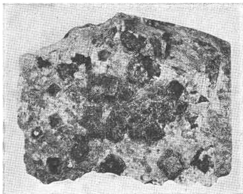
Fig. 1. Photograph showing crude cubic and octahedral crystals of altered uraninite enclosed in darker thucholite.
