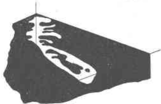
Fig. 5. Skeleton quartz crystal from Agate Pt. showing almost complete resorption. Only the ends of the axial plates are left.
