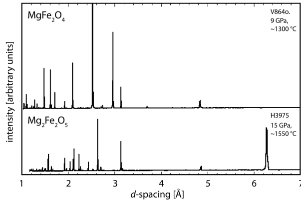
FIGURE 8. Comparison of powder X-ray diffraction patterns of \text{Mg}_2\text{Fe}_2\text{O}_5 and \text{MgFe}_2\text{O}_4 .
