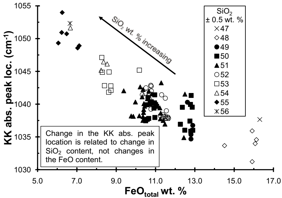
FIGURE A1. Plot of KK-abs. peak location vs. FeO total wt% of basaltic glasses. Data plotted are for 100 correlated spot analyses measured on 20 basaltic glass beads (Appendix 1) and symbols represent SiO 2 increments. Wavenumbers have an error of \pm 2 \text{ cm}^{-1} .
