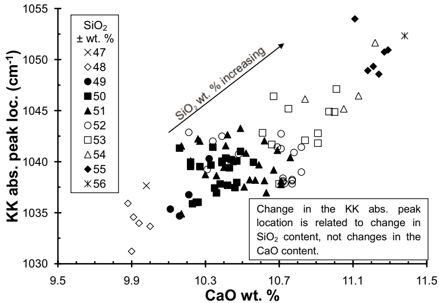
FIGURE A2. Plot of KK-abs. peak location vs. CaO wt% of basaltic glasses. Data plotted are for 100 correlated spot analyses measured on 20 basaltic glass beads (Appendix 1) and symbols represent SiO 2 increments. Wavenumbers have an error of \pm 2 \text{ cm}^{-1} .
