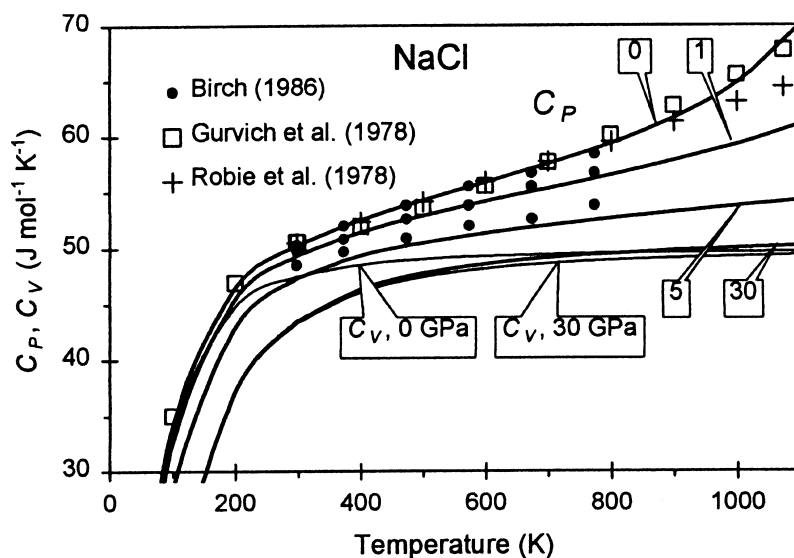
FIGURE 3. Heat capacity at constant pressure and constant volume, C_P and C_V , vs. T for rock salt. The thick, solid lines represent C_P calculated using SW EoS for 0, 1, 5, and 30 GPa isobars; the thin lines represent C_V at 0 and 30 GPa.
