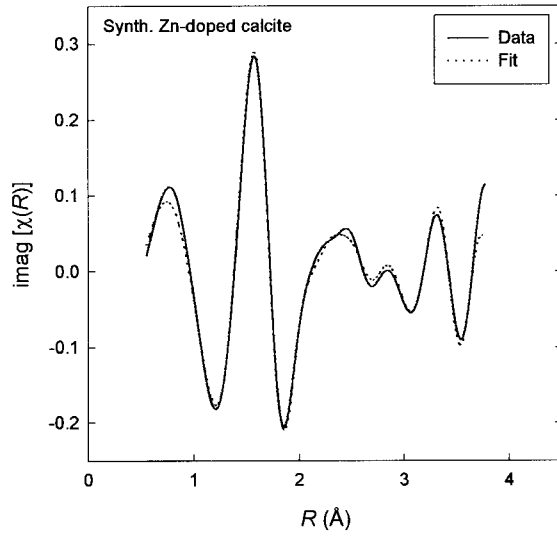
Figure 3. Fit of the imaginary \chi(R) function (dashed line) to raw data (solid line) for a synthetic Zn-doped calcite (945 ppm Zn).
