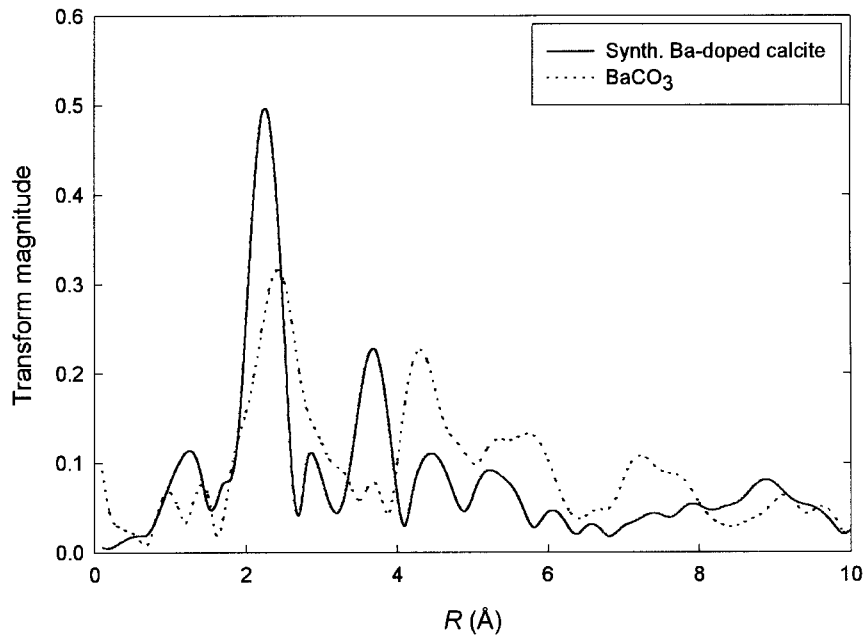
Figure 5. Fourier-transform magnitudes, uncorrected for phase shifts, of the synthetic Ba-doped calcite (solid line) and orthorhombic BaCO 3 (dashed line).
