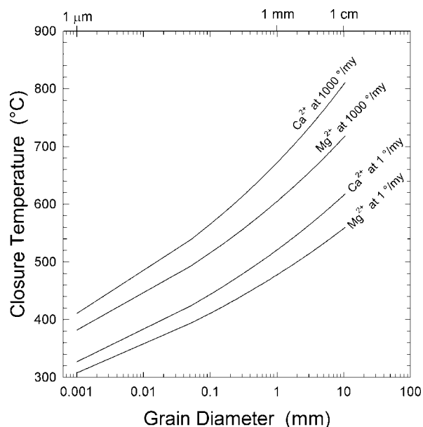
FIGURE 7. Closure temperature as a function of grain diameter (and cooling rate) showing the maximum temperatures required to homogenize a heterogeneous carbonate assemblage by diffusion of cations based on the experimental Arrhenius values for Ca and Mg diffusion.
