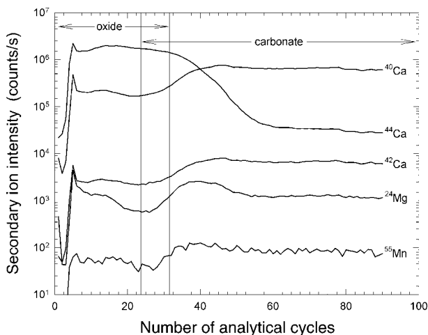
FIGURE 1. Ion microprobe depth profiles for Ca diffusion in calcite as a function of analysis cycle for sample cc600a annealed at 600 °C showing the concentration of ^{24}\text{Mg} , ^{40}\text{Ca} , ^{42}\text{Ca} , ^{44}\text{Ca} , ^{55}\text{Mn} , and the limits on the inferred position of the interface between the thin film coating and the calcite substrate (modified from Fisler and Cygan 1998).
