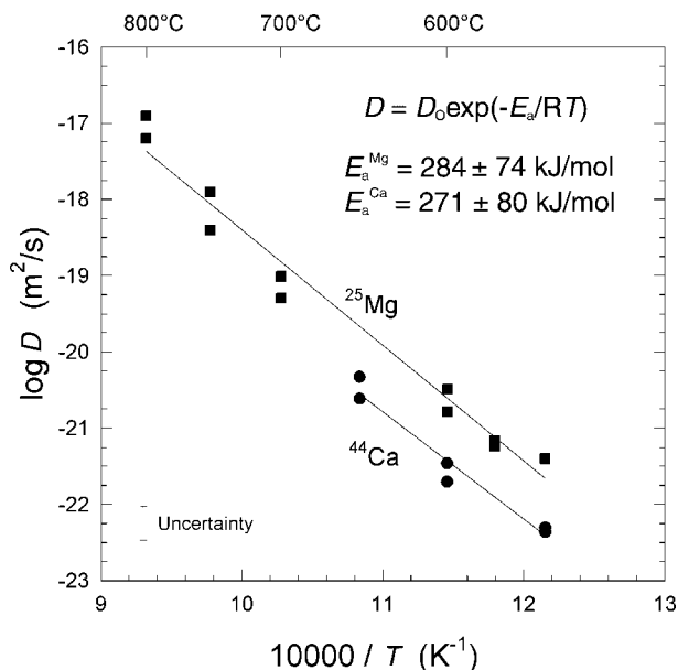
FIGURE 5. Arrhenius plot for Ca self-diffusion and Mg tracer diffusion in calcite. The error bar shown in the lower left represents the cumulative uncertainty in the final measurement based on the propagation of errors associated with the curve fitting and profile-to-profile variation.
