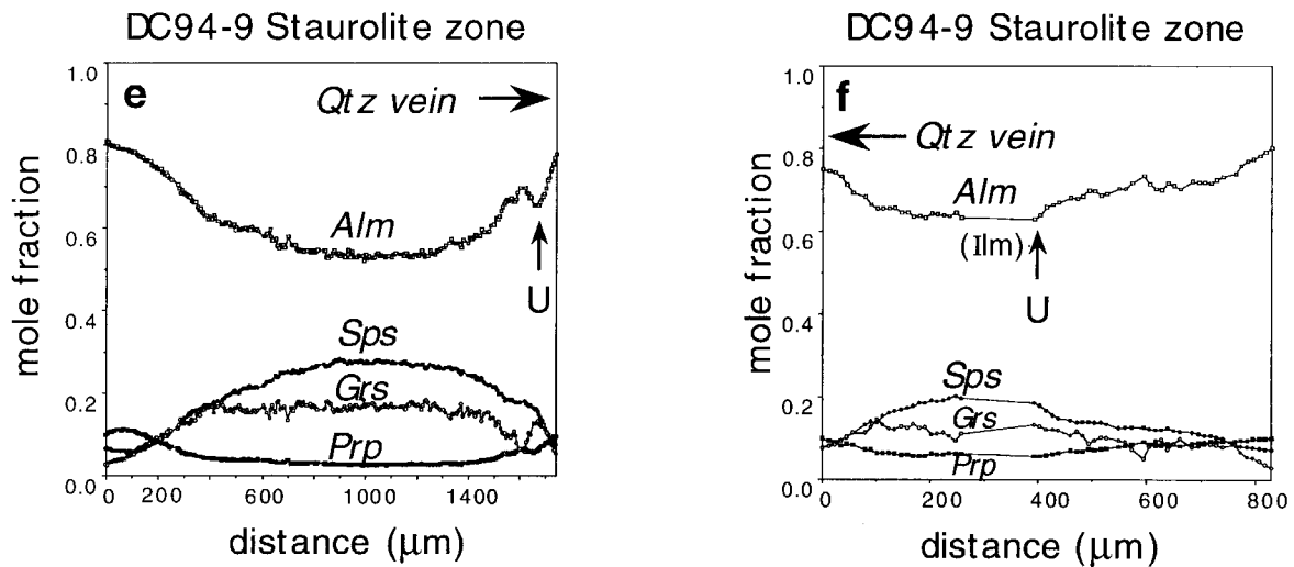
FIGURE 3. Staurolite-zone sample DC94-9. (a) Reaction texture between garnet and quartz vein. A fluid-inclusion-filled zone occurs at the contact between garnet and vein, an area free of quartz inclusions. Zoning profile given in e. Field of view = 2 mm. (b) View of inclusion-rich zone at higher magnification. Note the distribution of fluid inclusions in numerous linear zones perpendicular to the garnet-vein contact. Field of view = 0.75
