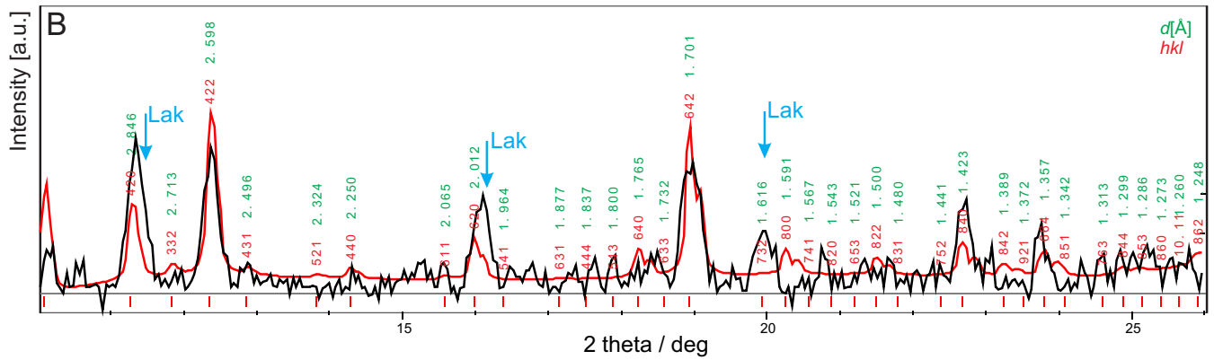
Appendix 2: Figure 4. A- the calculated diffraction pattern of garnet with 42% elbrusite-(Zr) end-member (green line, Table 1, analysis 7, a = 12.7456(9) Å on the basis of single-crystal diffraction data) and the experimental powder diffraction pattern obtained for garnet with 43% elbrusite-(Zr) end-member (Table 1, analysis 13); B- results of Rietveld refinement. Because of the high degree of metamictization of this garnet only the strongest lines are visible on the experimental curve. As a matter of record, a = 12.75(3) Å was determined. Blue arrows show the strongest lines of lakargiite (Lak).
