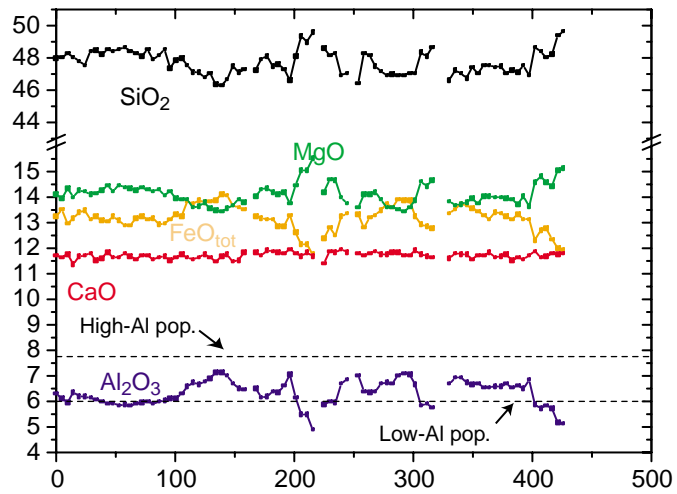
f) Granodioritic xenolith
