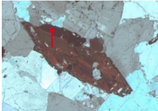
f) Granodioritic xenolith
