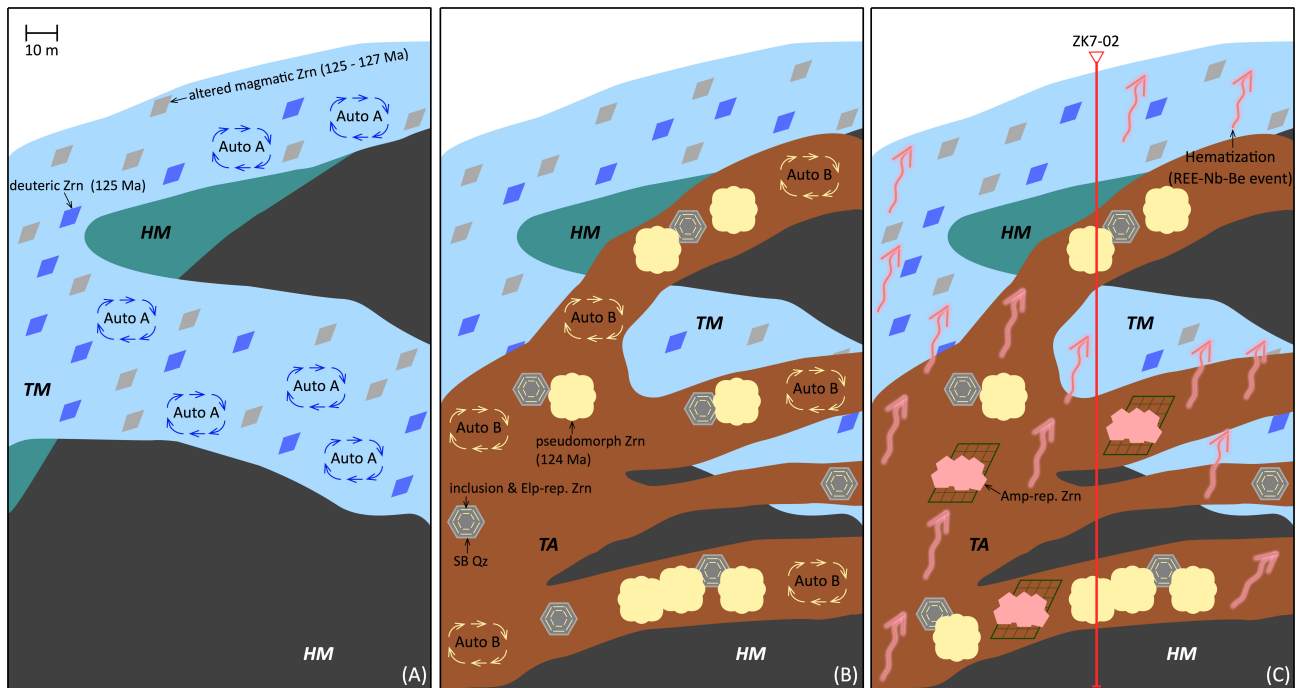
A schematic diagram illustrating the emplacement sequences (A - C), autometasomatism, and hematization (REE-Nb-Be-mineralizing event) of the Baerzhe miaskitic-agpaitic complex, and their impact on multi-stage metasomatic zircon crystallization. Abbreviations: HM = hypersolvus miaskitic granites, namely the fine-grained and porphyritic hypersolvus phases; TM = transsolvus miaskitic granite; TA = transsolvus agpaitic granite; Auto A = autometasomatism in the transsolvus miaskitic granite; Auto B = autometasomatism in the transsolvus agpaitic granite.
