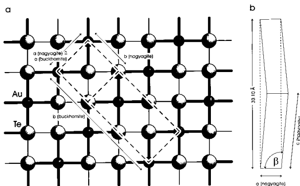
FIGURE 4. (a) A theoretical ordering scheme within the gold-tellurium layer for nagyagite based on the ratio Au:Te = 1:2 and considering the often observed tripled cell parameter a . The average cell of the structure model with Te and Au at one position used during the present work ( a_{\text{nagyagite}} and b_{\text{nagyagite}} ) is indicated. Assuming structural analogies between nagyagite and buckhornite, the cell parameters given by Francis et al. (1992) for buckhornite ( a_{\text{buckhornite}} and b_{\text{buckhornite}} ) correspond to those of a theoretical and ordered gold-tellurium layer in nagyagite. (b) Multiple twinning on (001) results in an orthorhombic symmetry for nagyagite with doubled cell parameter c .
