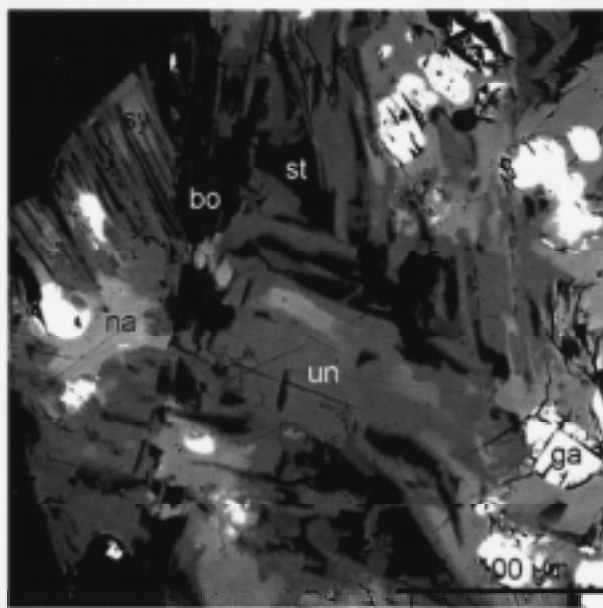
FIGURE 1. Complex assemblage of synthetic nagyagite (na) rimmed by the unknown phase "X" (un) and intergrown with sylvanite (sy), stuetzite (st), boulangerite (bo), and galena (ga).
