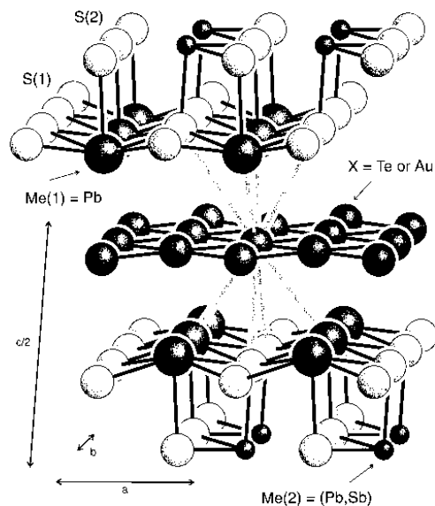
FIGURE 3. The connection between the \text{SnS} -archetype layers and the gold-tellurium layers in the average crystal-structure of nagyagite: the eight weak bonds are shown for one X = (\text{Au,Te}) atom only (program ATOMS, Dowty 1997).
