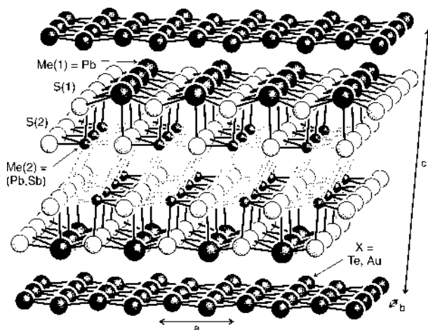
FIGURE 2. The average crystal-structure of nagyagite formed by \text{SnS} -archetype layers \text{Pb}(\text{Pb,Sb})\text{S}_2 separated by a planar pseudosquare net of gold and tellurium atoms (program ATOMS, Dowty 1997).
