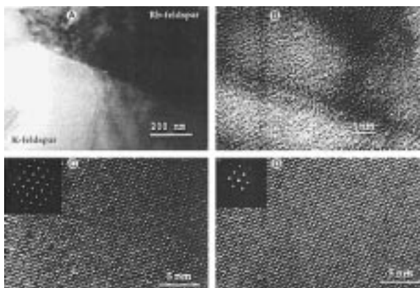
FIGURE 3. TEM micrographs: (A and B) the interface between rubicline and microcline; (C and D) high-resolution “lattice” image and SAED pattern of rubicline and microcline, respectively.
